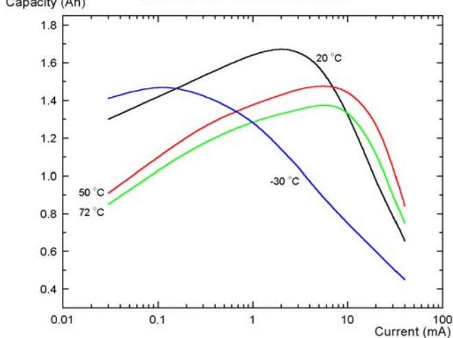
CAPACITY vs. CURRENT
