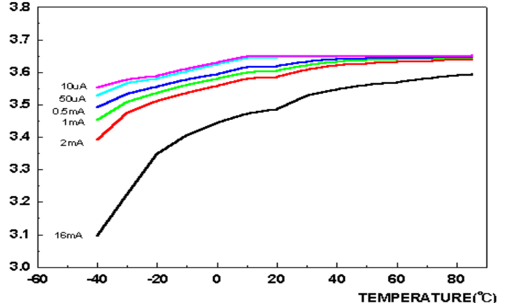
Voltage(V) TEMPERATURE vs. OPERATING VOLTAGE
